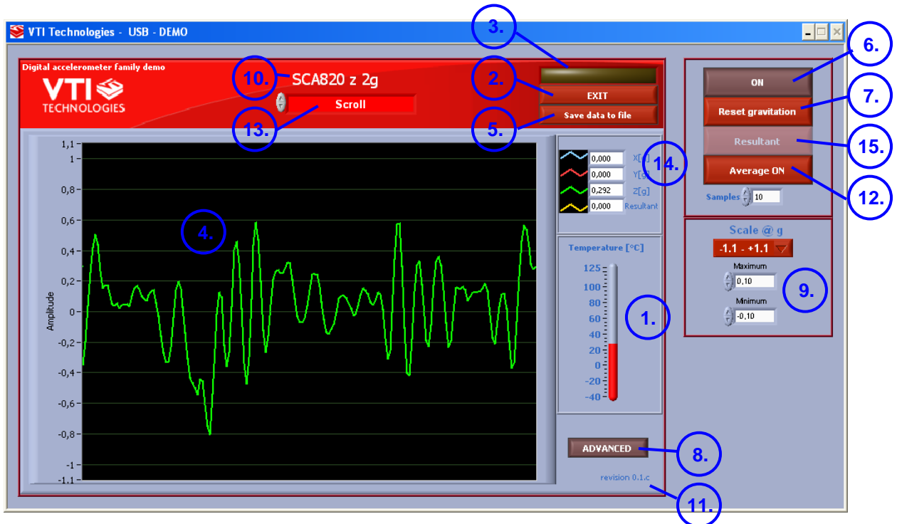
Figure 2. SCA8X0-21X0-31X0 DEMO KIT Graphical User Interface
