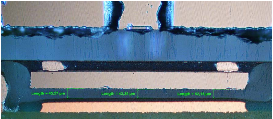
Figure 13. Gap between the component and the PWB.
