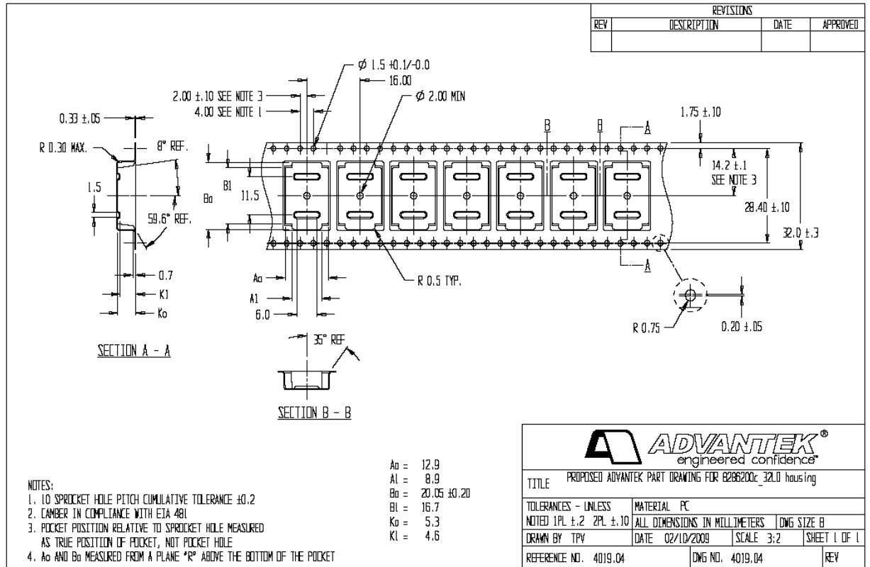
Figure 3: Packing tape dimensions for the DIL-32 Package. Dimensions are in millimeters [mm].
